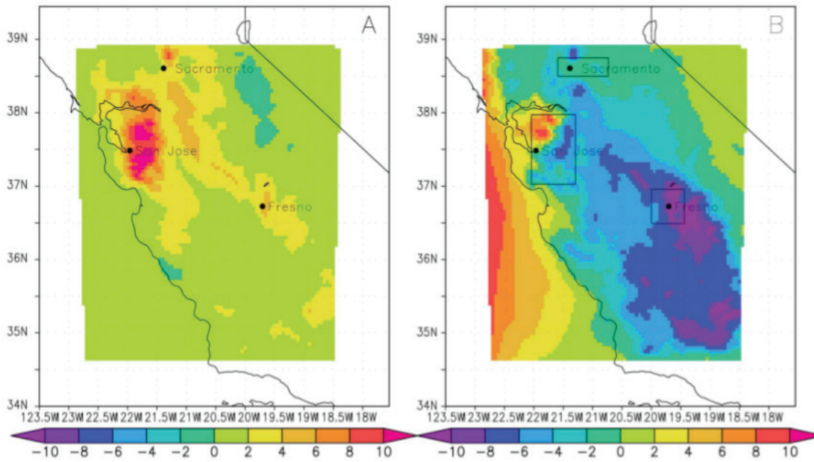
Change in ozone concentration (3 p.m. local time) for (a) combined climate effects; and (b) including emissions reductions. For the Bay Area, increases in ozone concentration mostly increase, except in the far southeast portions of the region, where reduced emissions dominate the increases due to climate factors. Source: Steiner et al. 2006
