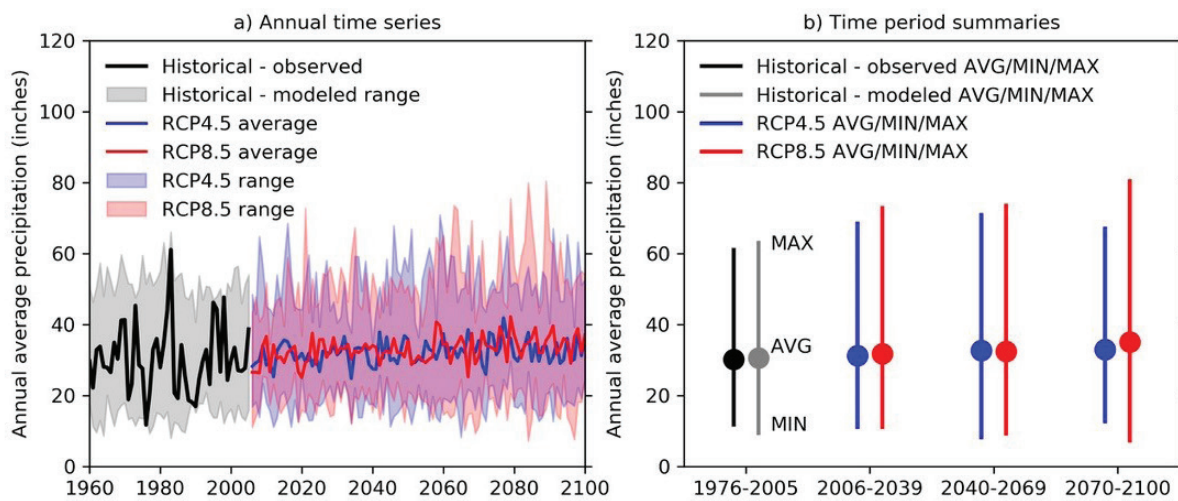
Observed historical (black), modeled historical (grey), and projected future (RCP4.5 - blue, RCP8.5 - red) annual average precipitation over the Bay Area. (a) Annual time series of data (future projections begin in 2006), with solid lines representing observed annual mean in the historical period and model-averages in the future. Shading represents the spread across models. (b) Summary of multi-year average (circles) and spread (vertical lines) across four time periods: 1976-2005 (historical), 2006-2039 (early-21st century), 2040-2069 (mid-21st century), and 2070-2100 (late-21st century). Unit is inches.
